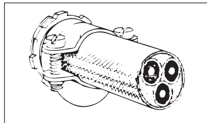
Installation type (cordon flexible)
