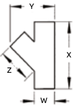
Left-hand wye
