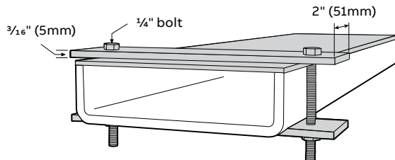
Heavy-duty cover clamp
