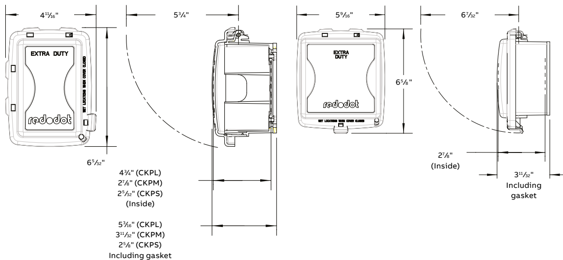
Single-gang (CKPM) – dimensions
