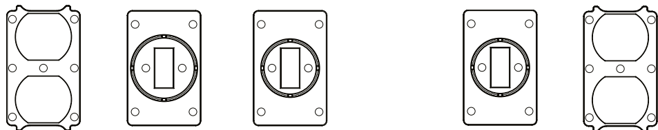
Single-gang (CKPM) – dimensions
